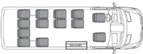
13 Passengers – ELB3
