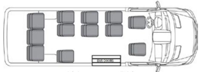
12 Passengers – ELB2
