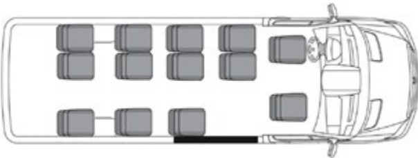
13 Passengers – EL1
