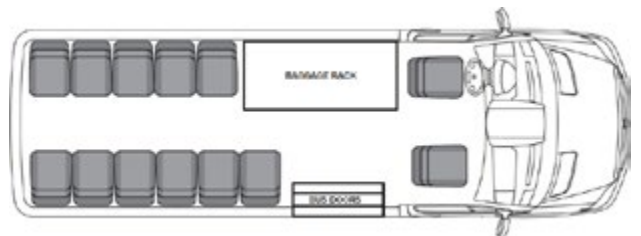
13 Passengers – ELB4
