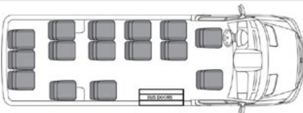
15 Passengers – ELB5
