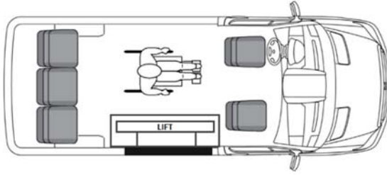
Ford Transit 150 Passenger Van Side Lift, 5 Passengers, 1 Wheelchair RWBS2
