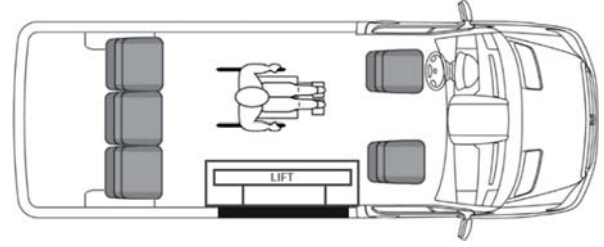
Ford Transit 350 Passenger Van ( More Cargo Room ) Side Lift, 5 Passengers, 1 Wheelchair LWBS1
