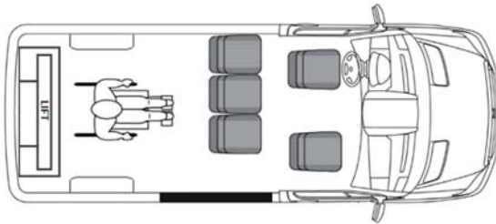
Ford Transit 150 Passenger Van Rear Lift, 5 Passengers, 1 Wheelchair RWBR1
